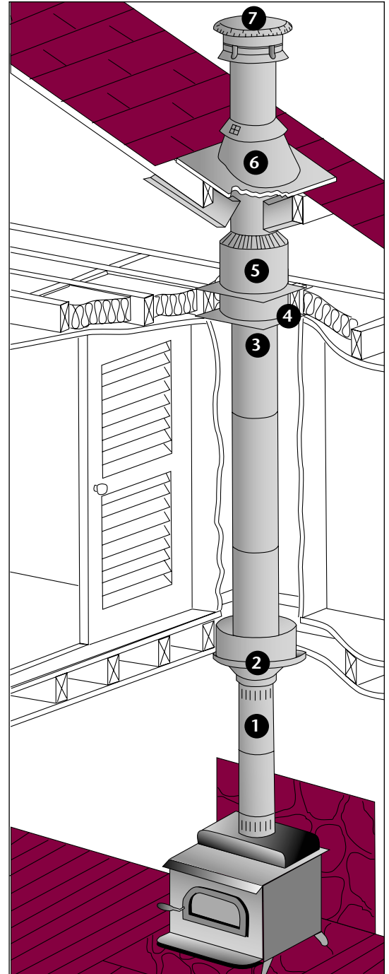
Interior installation of a Secure Temp™ASHT+ high-temperature chimney on a stove using a finishing support.
